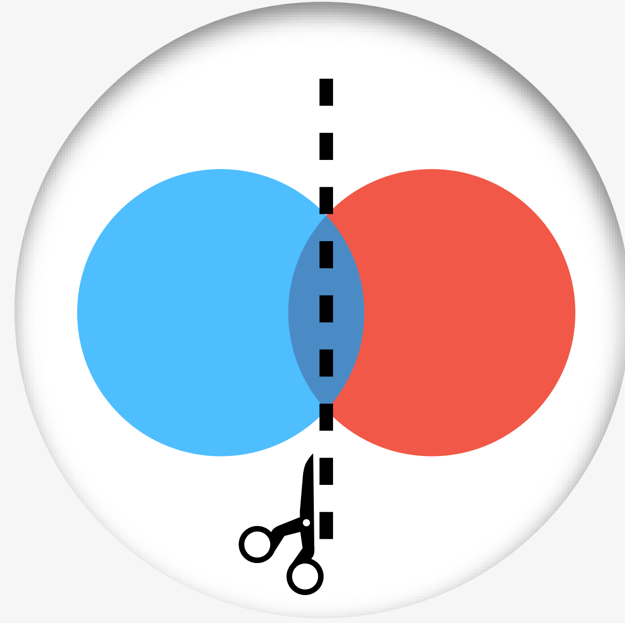
Discretization Error
