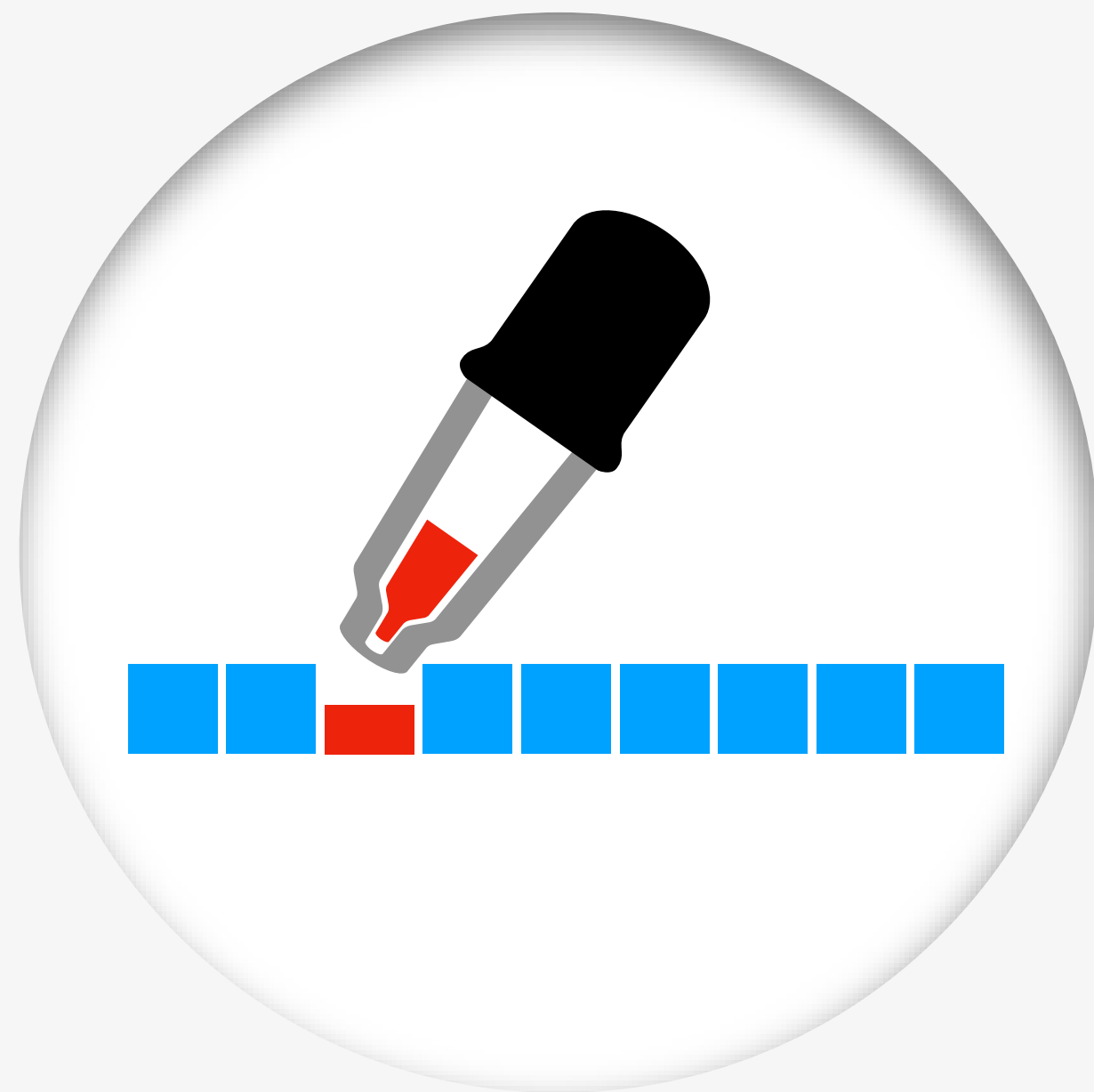
Sampling Error
